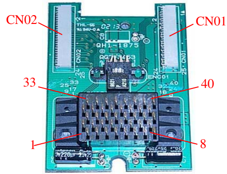
Figure 3-2 Carriage Board
