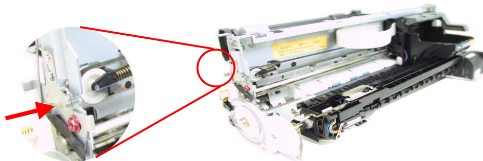
Figure 1-2 Code Strip
